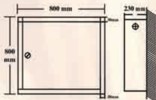
FRONT SIDE Surface Type Model SS7000
