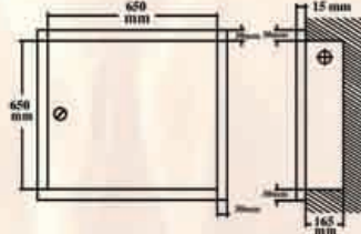
FRONT SIDE Recess Type Model SS4500
