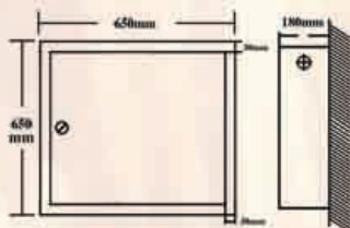
FRONT SIDE Surface Type Model SS3500
