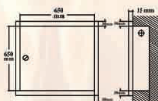
FRONT SIDE Recess Type Model SS3500
