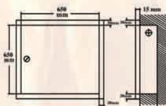
FRONT SIDE Recess Type Model SS450
