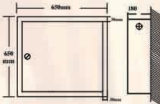
FRONT SIDE Surface Type Model SS450
